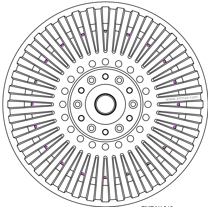
EMRAX 348 Front view
